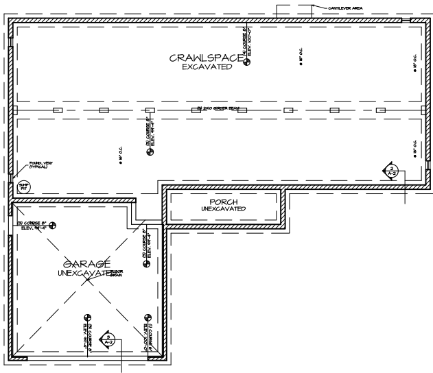
FOUNDATION PLAN A-2 SCALE: 1/4"=1'-0"
